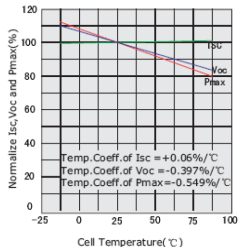
Temperatur dependence of Isc, Voc and Pmax
